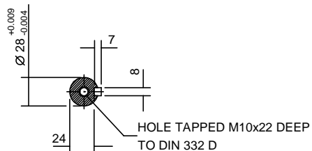
SECTION ON 'X'
